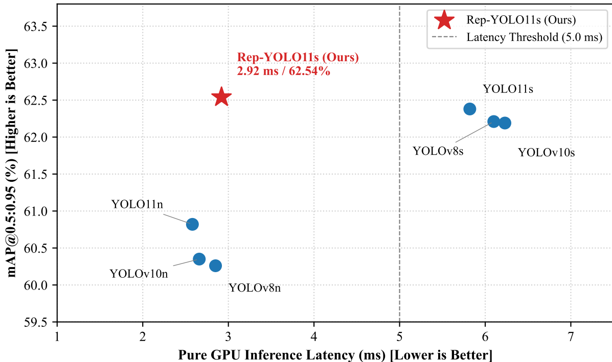
Efficiency Frontier: Accuracy vs Inference Latency
